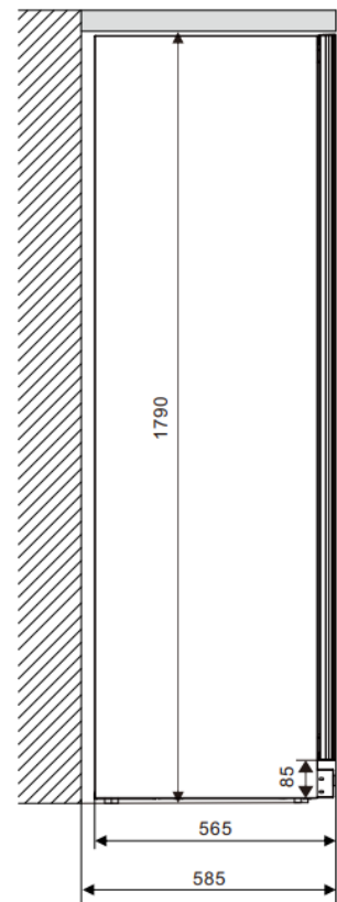
Side View
