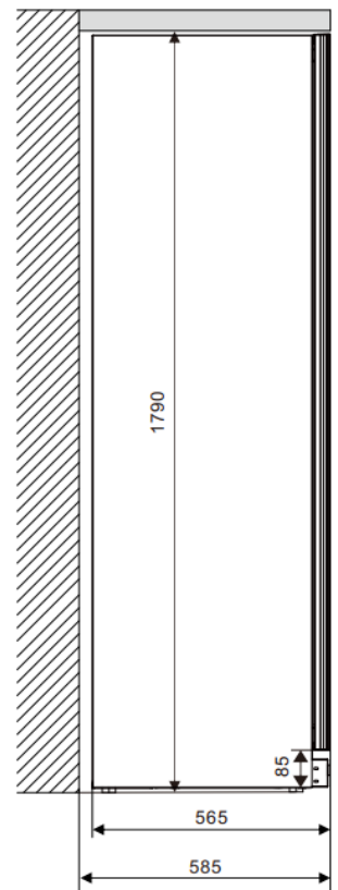
Side View
